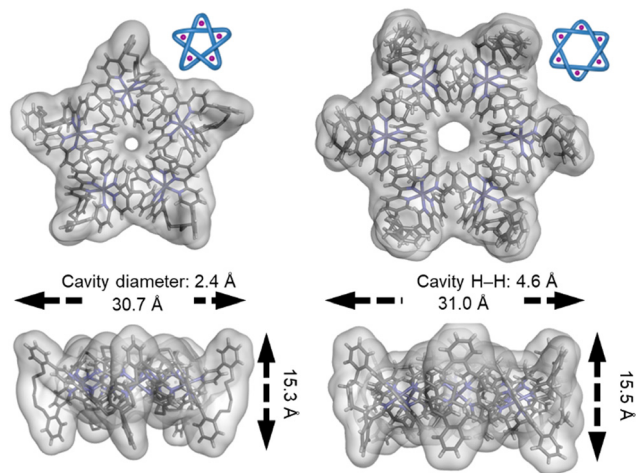
Fig. 32 The central cavities of pentafoil knot \text{Fe}_5^{II}\mathbf{20} and Star of David catenane \text{Fe}_6^{II}\mathbf{21} , visualized by overlaying the crystal structures with the solvent-accessible surfaces. 55,56,139 Reworked from ref. 139 by a CC-BY license.
