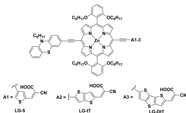
Fig. 34 Chemical structure of LG-5, LG-tT and LG-DtT.
