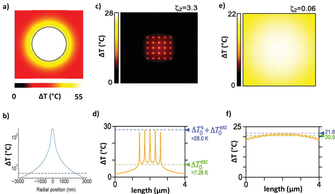
Fig. 6 (a) Equilibrium distribution of the temperature increase around an Au NP with a diameter of 100 nm irradiated with \lambda = 530 nm. Adapted with permission from ref. 143. Copyright 2010 American Chemical Society. (b) Temperature profile around an irradiated Au NP with a diameter of 150 nm (adapted from ref. 147. This work is licensed under a Creative Commons Attribution 4.0 International License). (c and d) Temperature distribution throughout a finite-size square lattice of NPs, uniformly illuminated ( p = 300 nm, d = 15 nm, N = 5 \times 5 , and I = 5.7 \times 10^9 W m ^{-2} ). Reprinted (adapted) with permission from ref. 146. Copyright 2013 American Chemical Society. (e and f) Temperature distribution throughout an infinite and periodic square lattice of NPs illuminated by a uniform circular beam ( p = 150 nm, d = 40 nm, D = 6 \mu m, and P = 2 mW). Reprinted (adapted) with permission from ref. 146. Copyright 2013 American Chemical Society.
