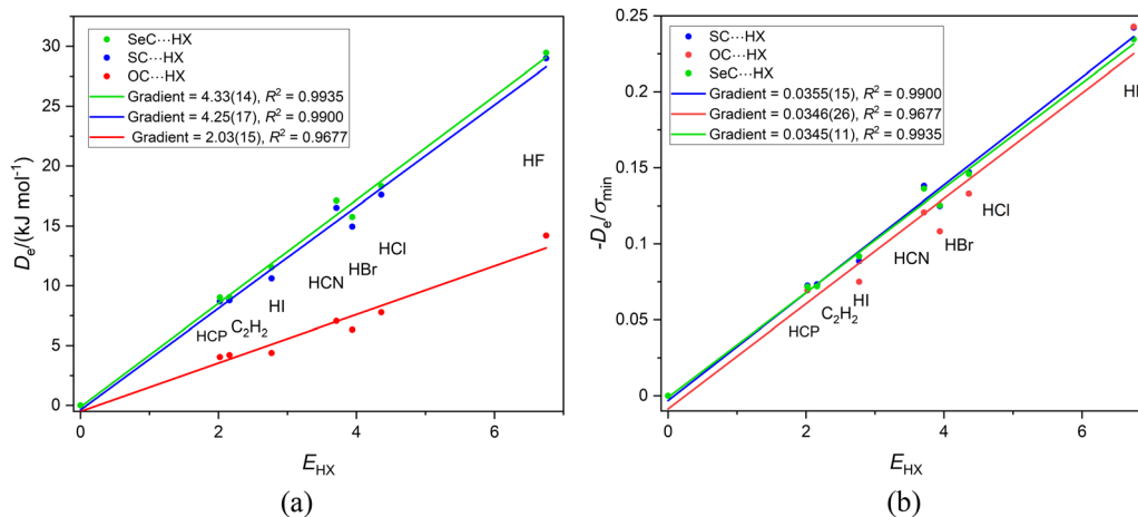
Fig. 1 (a) A plot of D_e versus E_{HX} for the series OC \cdots HX , SC \cdots HX and SeC \cdots HX for X = F, Cl, Br, I, C \equiv N, C \equiv CH and C \equiv P . (b) A plot of D_e/\sigma_{min} for the same series.
