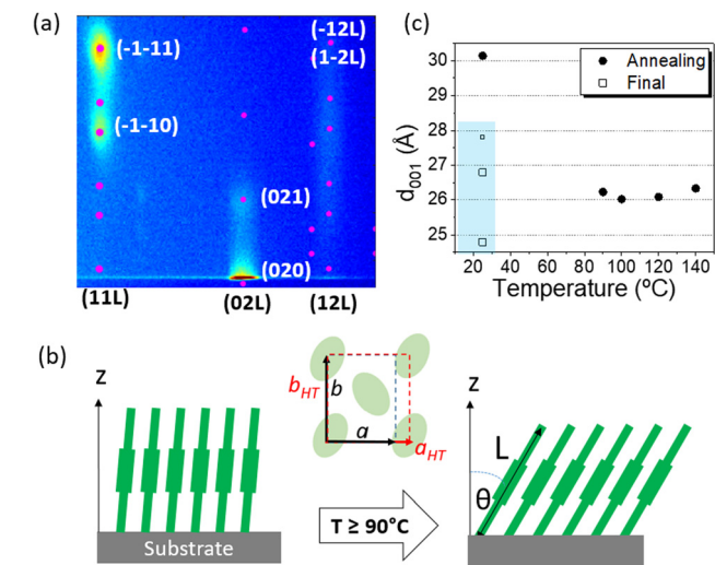
Fig. 2 (a) 2D diffraction pattern measured at 90 °C and simulated pattern (pink dots) for the HTP structure with the unit cell parameters given in Table 1. (b) Sketch illustrating the main changes involved in the structural transition from the SIP to the HTP structure with annealing temperature: tilting of the molecules and expansion of the a -lattice parameter. (c) Interplanar spacing at different temperatures extracted from the (001) peak. After annealing, the film was cooled down and measured at 25 °C (final); the values appear with square symbols, the smaller size of one of them indicates the lower intensity of the corresponding peak (see Fig S2 in ESI†).
