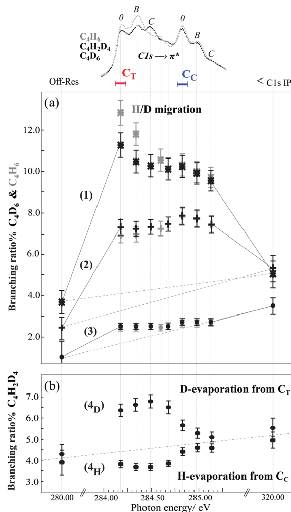
Fig. 4 Branching ratio as a function of the photon energy plotted in (a) for pathways (1) to (3) in C_4H_6 and C_4D_6 , and in (b) for pathways (4 D ) and (4 H ) in C_4H_2D_4 . The dashed line indicates the thermodynamical rate of dissociation determined from off-resonance excitation below and above the C 1s ionization threshold. The branching ratios for double-coincidence events are calculated using two ions, each of which have a detection efficiency of 40%. An overall contribution of about 5% false coincidence events to each data set is estimated. The reduction for identical ion coincidences (pathway 2), due to the electronics system dead-time of 20–25 ns, is corrected with a factor of 1.85. The resulting error in the branching ratios for a 10% contribution is about \pm 0.5\% .
