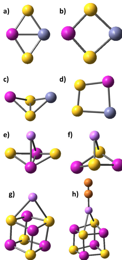
Fig. 1 Cation binding to cobalt sulphides and persulphide: (a) planar rhombic disulphide \text{CoS}_2\text{--Zn} with \text{Co--Zn} bond, \text{C}_{2v} symmetry and notation of bonding scheme \text{CoZn}(\mu\text{--S})_2 ; (b) rhombic disulphide \text{CoS}_2\text{--Zn}^{2+} with \text{C}_{2v} symmetry; (c) non-planar rhombic persulphide \text{Co}(\text{S}_2)\text{--Zn}^{2+} with \text{C}_s symmetry; (d) rhombic planar persulphide \text{CoZn}(\text{S}_2) with \text{C}_s symmetry and side-on bonding of disulphur; (e) \text{Li}^+, \text{e}^- binding to rhombic \text{Co}_2\text{S}_2 cluster with \text{Co--Li} bond formation; (f) \text{Li}^+ binding to \text{Co}_2\text{S}_2 via \text{S--Li} bond formation; (g) \text{Li}^+ binding to \text{Co}_4\text{S}_4 ; (h) \text{N}_2 adsorption to the \text{Co}_4\text{S}_4\text{--Li}^+ cluster. Colour legend: Cobalt atoms are red, zinc atoms – blue, lithium ions – small pink balls, sulphur atoms – yellow, nitrogen atoms – orange.
