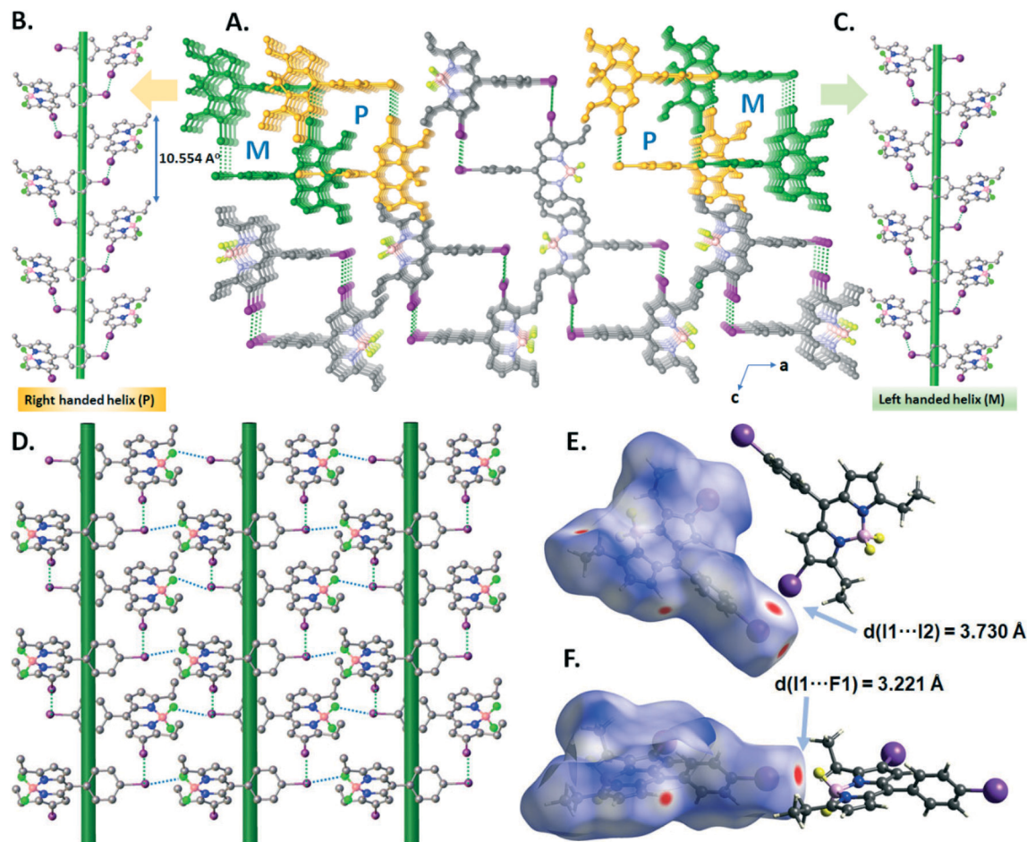
Fig. 6 (A) View of the 3D supramolecular network showing P and M helicity in the crystal packing in B4. (B) and (C) Illustrations of P and M helices. (D) A 2D halogen-bonded layer formed by I...F (blue dotted lines) and I...I (green dotted lines) XB interactions showing their d -norm mapped Hirshfeld surface representations (E and F).
