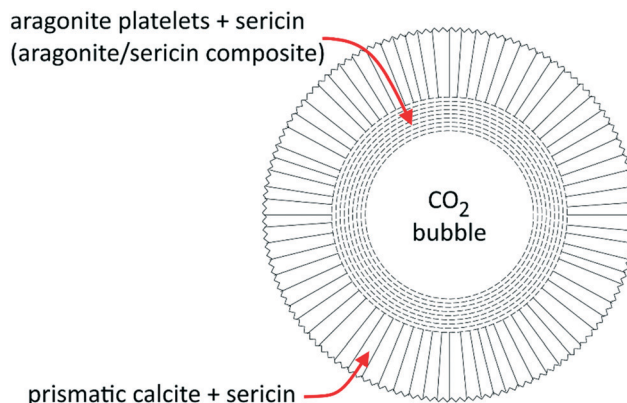
Fig. 5 Structure of the spherulite grown in the presence of sericin. Around the core cavity (a \text{CO}_2 bubble) aragonite and calcite grow in concentric shells. Modified from Pastoro and Aquilano. 34
