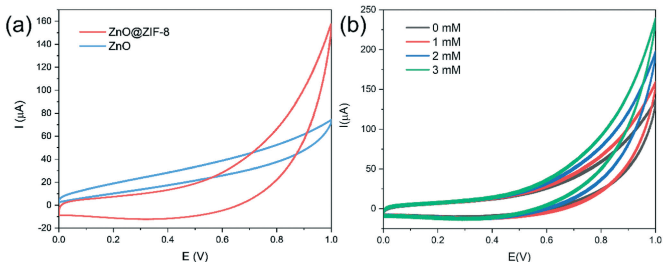
Fig. 5 (a) Cyclic voltammograms of the ZnO nanorod arrays and the ZnO@ZIF-8 nanorod arrays in the presence of 1 mM \text{H}_2\text{O}_2 in PBS (0.1 M, pH 7.0) at a scan rate of 50 \text{ mV s}^{-1} ; (b) cyclic voltammograms of ZnO@ZIF-8 nanorod arrays in PBS including various concentrations of \text{H}_2\text{O}_2 at 50 \text{ mV s}^{-1} .
