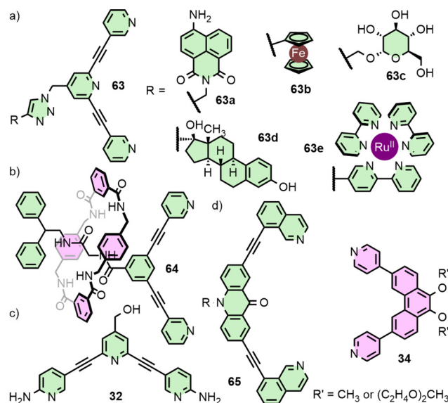
Fig. 12 (a) Exo-functionalisation of a tripyridyl ligand fragment via CuAAC chemistry with a variety of functional groups allowed access to a series of \text{Pd}_2\text{L}_4 cages in which the host-guest chemistry of the core cage was unaffected. (b) [2]Rotaxane 64 assembled into a \text{Pd}_2\text{L}_4 cage decorated with four mechanically interlocked macrocycle units. (c) ortho -amino groups appended to the coordinating pyridine units in 32 induce a helical twist in the resultant \text{Pd}_2\text{L}_4 cage, altering the host-guest properties compared to the unfunctionalised [\text{Pd}_2(\mathbf{17})_4]^{4+} parent system. (d) Geometrically matched ligand 65 and 34 assemble to form heteroleptic cage cis - [\text{Pd}_2(\mathbf{65})_2(\mathbf{34})_2]^{4+} , but only if R' = CH 3 .
