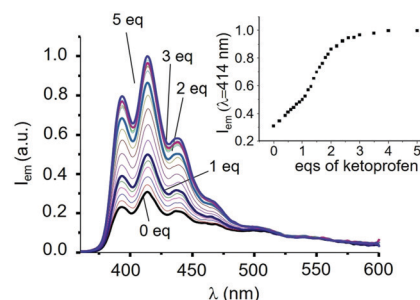
Fig. 1 Fluorescence emission spectra of L1 at pH 7 (0.001 M TRIS buffer) in \text{H}_2\text{O}/\text{EtOH} 50 : 50 (Vol : Vol) and (inset) emission intensity at 414 nm in the presence of increasing amounts of KP ( \lambda_{\text{exc}} = 340 nm, [\text{L1}] = 1 \times 10^{-5} M, 298 K).
