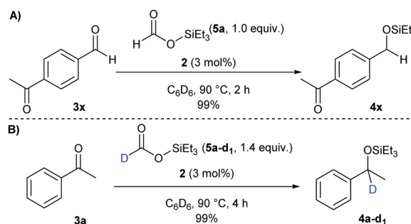
Scheme 4 Yields were determined by ^1H NMR with mesitylene as an internal standard. (A) Selectivity of the PN^{H}P -based ruthenium catalyst 2 for the transfer hydrosilylation of carbonyl groups (0.1 mmol scale). (B) Deuteriosilylation of ketones (0.1 mmol scale).
