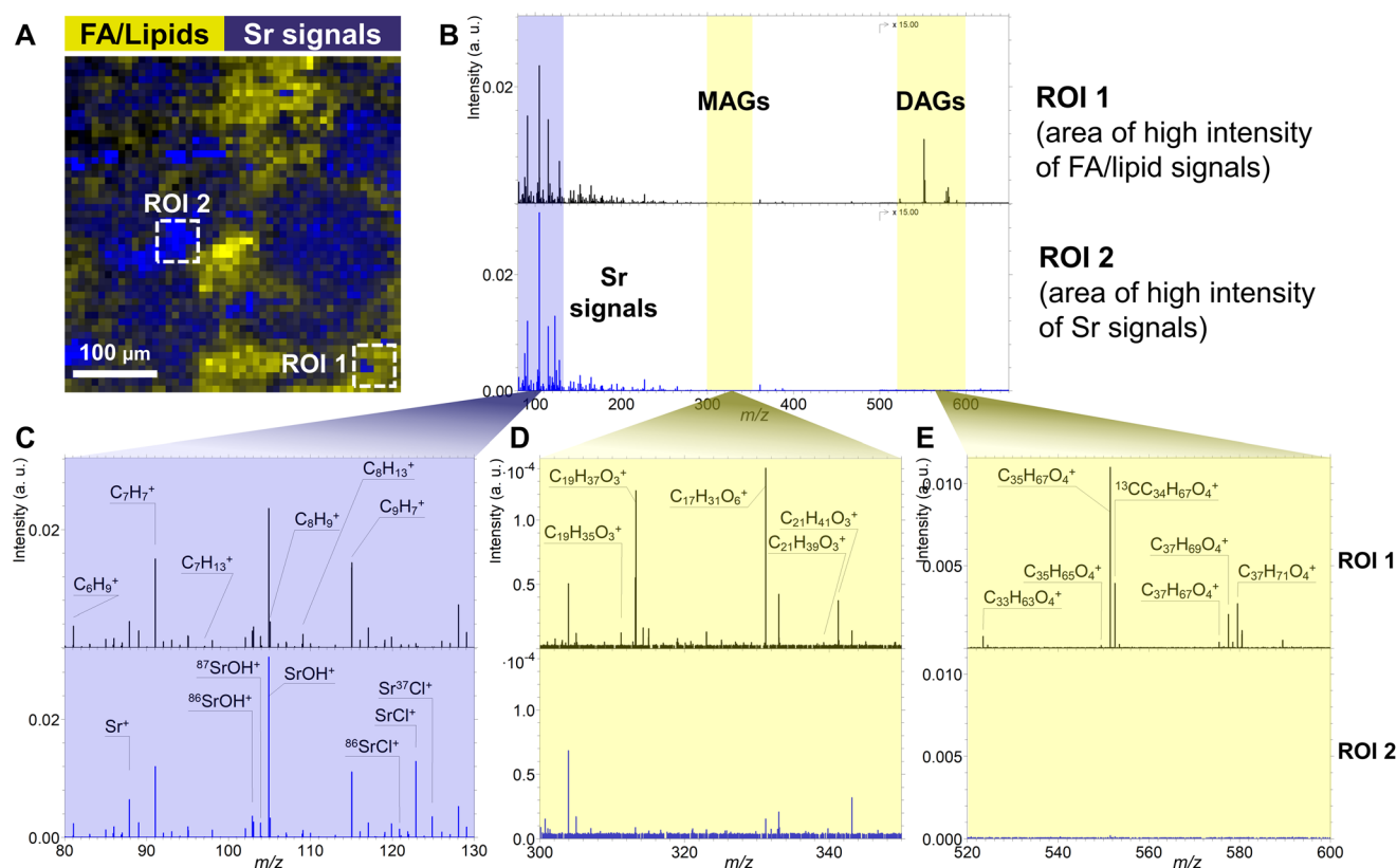
Fig. 6 Analysis of \text{Sr}^{2+} diffusion into rat bone marrow of osteoporotic rat using the OrbiTrap™ analyser. (A) Overlay of ion image of FA/lipid signals (yellow) and strontium signals (blue). Dotted boxes show the chosen areas of ROI 1 and ROI 2. ROI 1 is in an area with high intensity of fatty acid and lipid mass signals. ROI 2 is in an area with high intensity of strontium signals. (B) Positive mass spectra of ROI 1 and ROI 2 in a mass range of m/z 80–650. Mass ranges with signals from lipids (MAGs, DAGs) are marked in yellow. Mass range with strontium signals is marked in blue. (C) Detailed mass range of m/z 80–130 shows higher intensities of strontium signals in ROI 2 than in ROI 1. (D) Detailed mass range of m/z 300–350 shows higher intensities of mass fragments derived from MAGs in ROI 1 than in ROI 2. (E) Detailed mass range of m/z 520–600 shows higher intensities of mass fragments derived from DAGs in ROI 1 than in ROI 2. For comparison of the peak intensities, the spectra were normalised to the total counts (scale spectra by total counts). Identified peaks are listed in Table S3.† For Orbitrap imaging and spectral analysis, 20 keV \text{Ar}_{3000}^+ cluster primary ions were applied (positive ion mode, obtained with M6 Hybrid SIMS).
