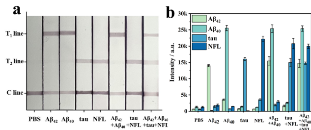
Fig. 7 Specificity evaluation of the SERS-LFA detection method. (a) Photographs of test strips for detecting different AD biomarkers at 10 μg mL -1 . (b) Raman intensities at 1079 cm -1 and 1330 cm -1 on the T line of the test strip. The error bars represent the average results of three measurements.
