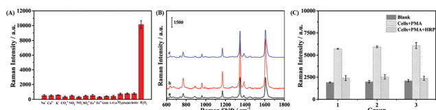
Fig. 5 (A) SERS response of TMB containing the \text{Fe}_3\text{O}_4@\text{Ag} NPs to the reaction of various interfering species: anions (1 mM for \text{CO}_3^{2-} , \text{NO}_2^- , \text{NO}_3^- , and \text{SO}_4^{2-} ), cations (1 mM for \text{Na}^+ , \text{K}^+ , \text{Ca}^{2+} , \text{Fe}^{2+} , and \text{Fe}^{3+} ), thiols (1 mM for GSH and L-Cys) and oxidative species (50 \mu\text{M} for ^1\text{O}_2 , \text{ONOO}^- , \text{ROO}^\bullet , and \text{H}_2\text{O}_2 ). (B) SERS spectra of TMB catalyzed by \text{Fe}_3\text{O}_4@\text{Ag} NPs with B16 cells (curve a), the cells after being treated with PMA (curve b), and the cells treated with HRP in advance of PMA stimulation (curve c), respectively. (C) The corresponding histogram of the change in the SERS intensity of the band at 1611\text{ cm}^{-1} in Fig. 5B from the three parallel groups of B16 cells.
