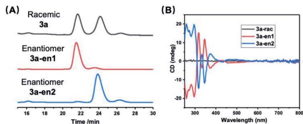
Fig. 5 Enantioseparation and characterization of chiral \text{Au}_{13} nano-clusters: (A) chromatogram showing the enantioseparation of rac - 3a by chiral HPLC using UV-vis detection at 350 nm; (B) CD spectra of the two chiral enantiomers separated by HPLC and rac - 3a for comparison.
