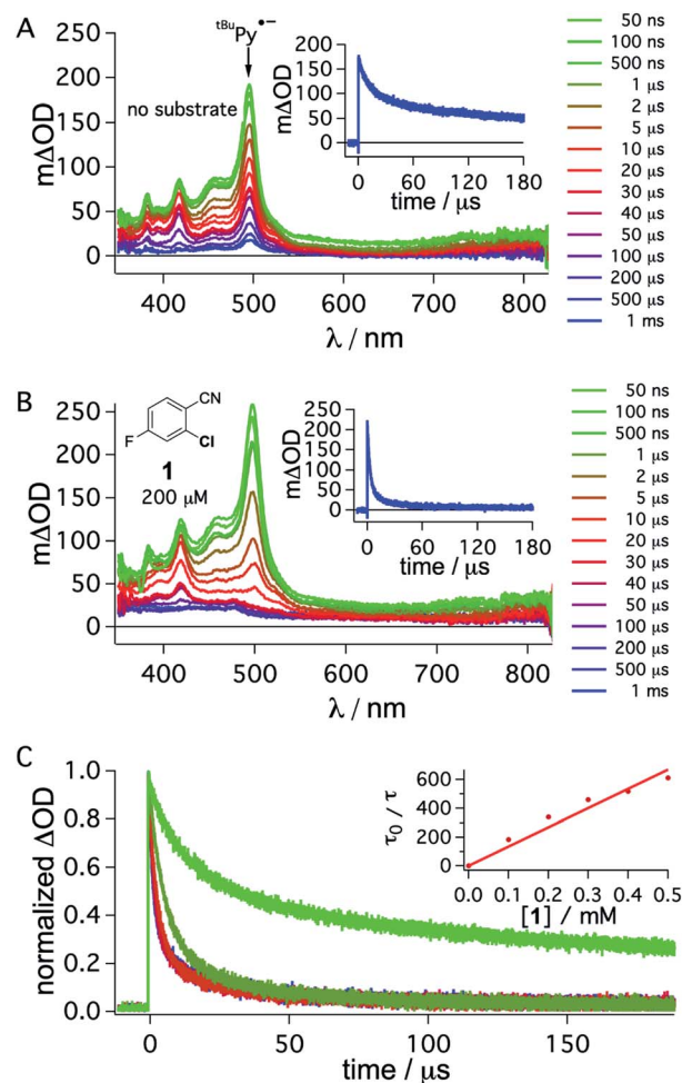
Fig. 5 Transient absorption spectra obtained after direct 355 nm excitation of {}^1\text{tBuPy}^+ (50 \mu\text{M} ) in de-aerated DMF in the presence of DMA (10 mM) (A), recorded at different delay times as indicated in the inset. Same experiment series performed on a solution containing substrate 1 (200 \mu\text{M} ) in addition to 50 \mu\text{M} {}^1\text{tBuPy}^+ and 10 mM DMA (B). Corresponding kinetic traces monitoring the decay of the {}^1\text{tBuPy}^+ signal at 495 nm over 180 \mu\text{s} in the respective solutions without and with substrate 1 are given in the insets of (A) and (B). {}^1\text{tBuPy}^+ disappears considerably more rapidly in the presence of substrate 1 (B) than in its absence (A). For clarity the most prominent spectroscopic feature of {}^1\text{tBuPy}^+ is marked by an arrow in (A). Kinetic traces at 495 nm (C) were monitored in the absence (bright green) and in the presence of different concentrations of 1 (0.1, 0.2, 0.3, 0.4, 0.5 mM). The Stern–Volmer plot for the shorter lifetime components obtained from biexponential fits to this data set is given in the inset of (C). A quenching constant of ca. 1.1 \times 10^9 \text{ M}^{-1} \text{ s}^{-1} is estimated for the electron transfer from {}^1\text{tBuPy}^+ to substrate 1 , based on an unquenched decay constant of 1.07 ms for {}^1\text{tBuPy}^+ . A 385 nm long-pass cut-off filter was installed between the sample and the flashlamp to prevent direct UV flashlamp excitation. Further details are in the main text and the ESI.†
