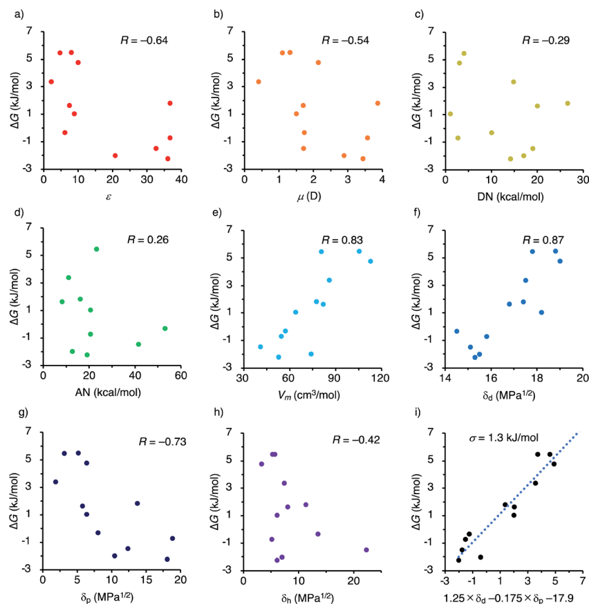
Fig. 4 \Delta G ( mer to fac ) plotted versus various solvent parameters and their correlation coefficient. (a) Dielectric constant \epsilon , 15a (b) dipole moment \mu (D), 15a (c) donor number DN (kcal mol -1 ), 15a,b (d) acceptor number AN (kcal mol -1 ), 15a (e) molar volume V_m (cm 3 mol -1 ), 14 (f–h) the Hansen solubility parameters, 14 (f) dispersion term \delta_d (MPa 1/2 ), 14 (g) dipole interaction term \delta_p (MPa 1/2 ), 14 (h) hydrogen bonding term \delta_h (MPa 1/2 ), 14 and (i) a prediction formula using \delta_d and \delta_p as explanatory variables.
