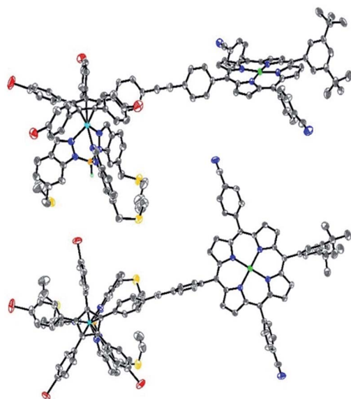
Fig. 5 Side view (top) and top view (bottom) of the molecular structure of monoporphyrinic ruthenium complex 13 . Thermal ellipsoids are drawn at 30% probability, and hydrogen atoms (except for B–H), solvent molecules and disordered atoms are omitted for clarity.
