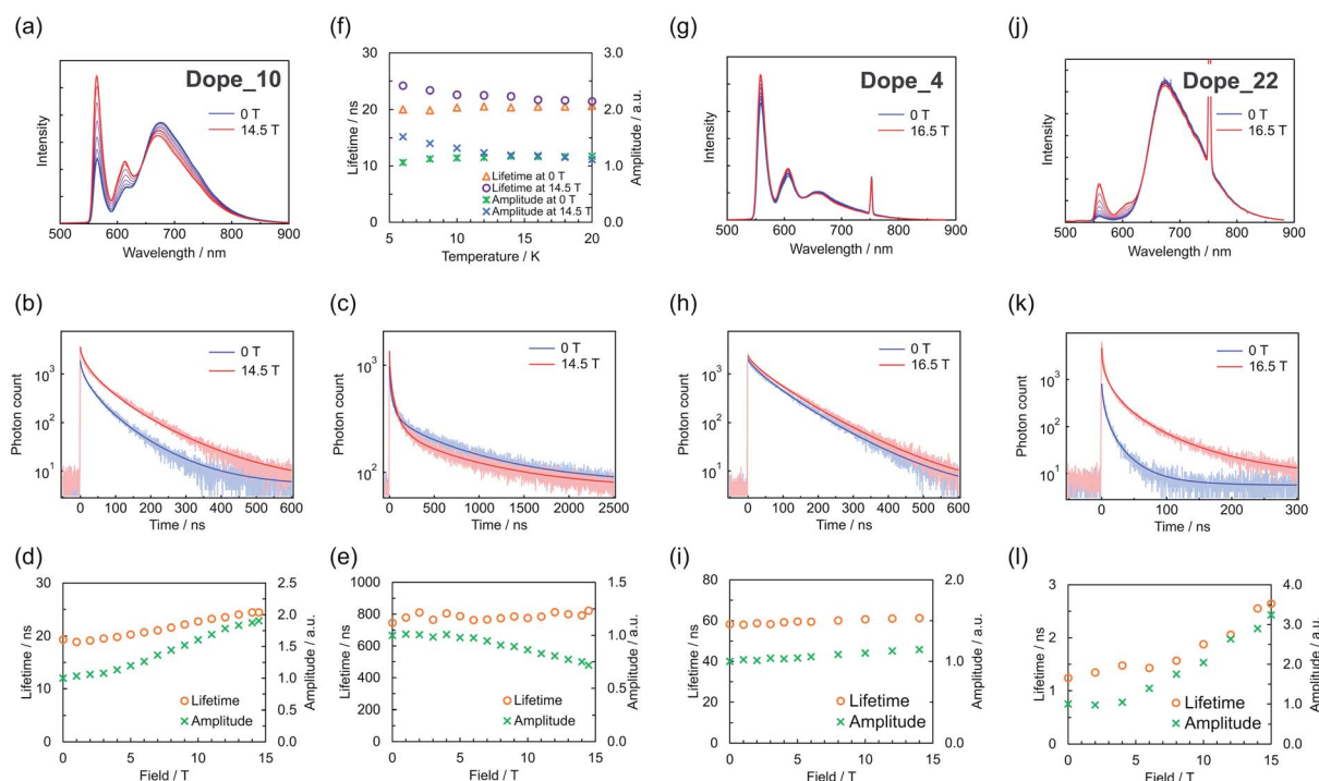
Fig. 2 (a–e) Emission spectra of Dope_10 at 4.2 K under magnetic fields of 0–14.5 T (a), emission decays and corresponding fits at 4.2 K under magnetic fields of 0 and 14.5 T at 563 nm (b) and 674 nm (c), and magnetic field dependences of lifetimes and amplitudes at 4.2 K at 563 nm (d; \beta = 0.59 ) and 674 nm (e; \beta = 0.88 ). (f) Temperature dependences of lifetimes and amplitudes at 563 nm under magnetic fields of 0 and 14.5 T ( \beta = 0.59 ). (g–i) Emission spectra of Dope_4 at 4.2 K under magnetic fields of 0–16.5 T (g), emission decays and corresponding fits at 4.2 K under magnetic fields of 0 and 16.5 T (h), and magnetic field dependences of lifetimes and amplitudes at 4.2 K (i) ( \beta = 0.78 ). (j–l) Equivalent results as in (g–i) for Dope_22 ( \beta = 0.41 ). Peaks at 750 nm are due to the excitation laser light ( \lambda_{\text{ex}} = 375 nm).
