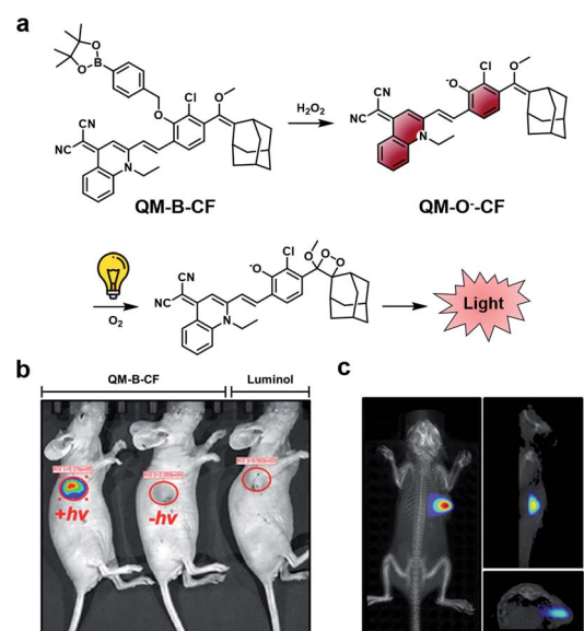
Fig. 6 Dual-lock strategy for CL emission enhancement. (a) Reaction scheme of QM-B-CF reacting with hydrogen peroxide to generate a stable fluorescent intermediate (QM-O - -CF), and following irradiation with light, the generation of a CL signal. (b) Comparison of CL signal from QM-B-CF with and without white light irradiation and Luminol (c) 3D image of QM-B-CF CL signal. Reproduced from ref. 45 with permission from Wiley-VCH Verlag GmbH & Co. KGaA, Weinheim, Copyright 2020.
