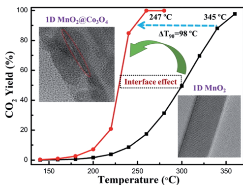
Fig. 11 Benzene oxidation activity tests of the 1\text{D MnO}_2\text{@Co}_3\text{O}_4 and 1\text{D MnO}_2 catalysts. Reproduced by Tang et al. 31 with permission from Elsevier.
