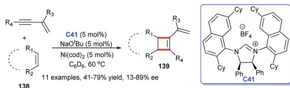
Scheme 45 The synthesis of cyclobutenes.
