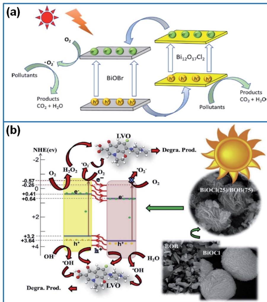
Fig. 8 (a) Schematic illustration for the transport and separation of the photo-induced electron–hole pairs and the degradation mechanism of BiOBr/Bi 12 O 17 Cl 2 composite. 159 Copyright 2020 Elsevier. (b) Degradation mechanism for removal of levofloxacin by using 3D flower-like BiOCl(25)/BOB(75) heterojunction photocatalysts. 160 Copyright 2020 Elsevier.
