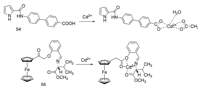
Fig. 19 Proposed binding mode of probes 54 and 55 with \text{Cd}^{2+} .
