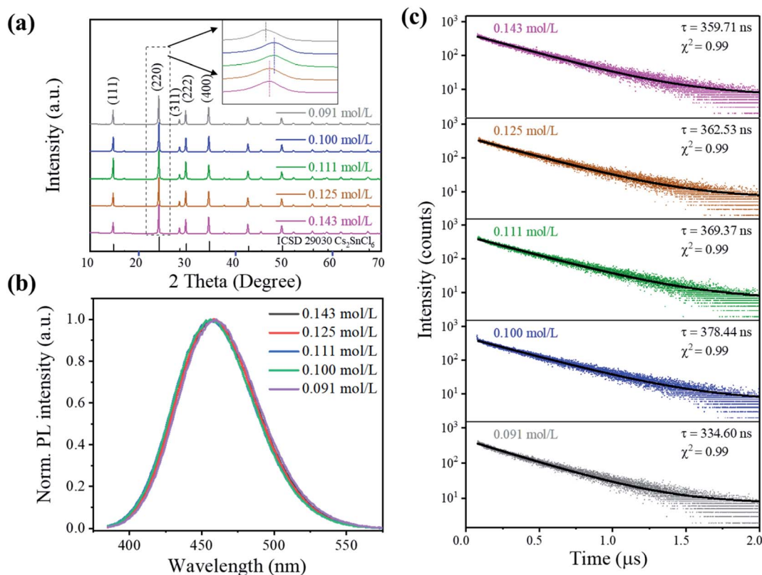
Fig. 2 Structure and luminescence properties of Cs 2 SnCl 6 :Bi 3+ synthesized at different precursor concentrations: (a) room-temperature XRD patterns and the enlarged (220) peak as an inset. (b) PL spectra of Cs 2 SnCl 6 :Bi 3+ ( \lambda_{\text{ex}} = 362 nm). (c) Time-resolved PL decay curve of Cs 2 SnCl 6 :Bi 3+ ( \lambda_{\text{ex}} = 375 nm and \lambda_{\text{em}} = 456 nm).
