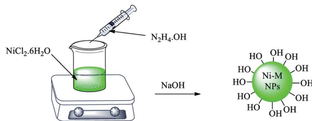
Scheme 1 Synthesis of nickel magnetic nanoparticles (Ni MNPs).
