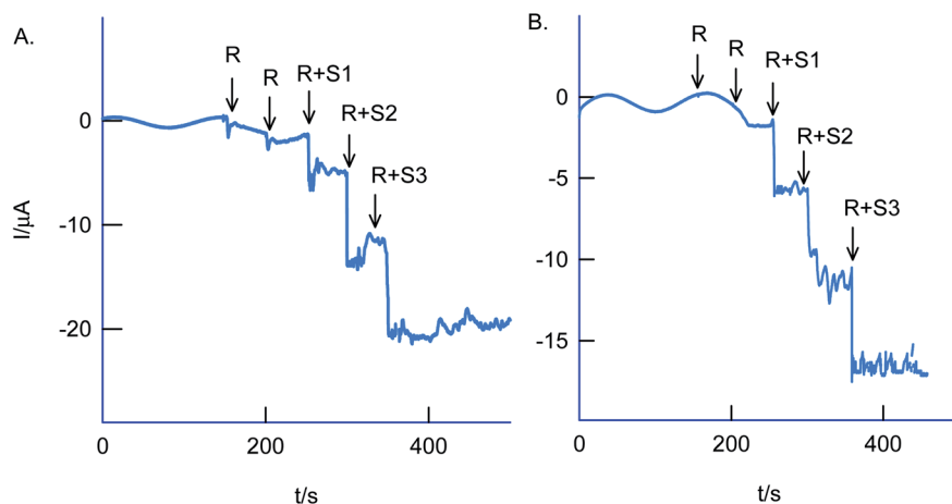
Fig. 14 Amperometric i - t based real sample analysis of Cr(VI) species in two industrial effluents samples using GCE/Nf-MWCNT@HQ modified electrode in pH 2 KCl-HCl solution. A four-time diluted test sample with pH 2 KCl-HCl was subjected for the analysis. E_{app} = 0.4 V vs. Ag/AgCl. R = real sample, R + S1–S3 = real + three different standard Cr(VI) concentration numbers, 1–3.
