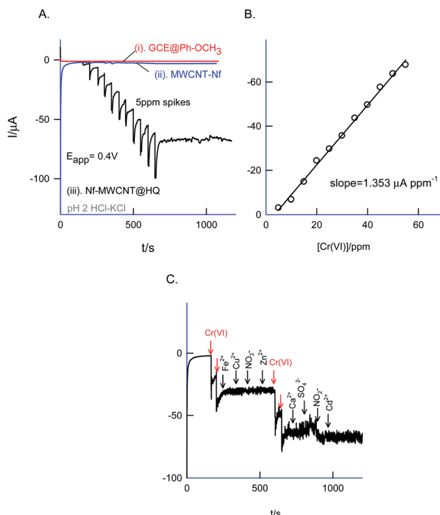
Fig. 13 (A) Comparative amperometric i - t responses of GCE@Ph-OCH 3 (curve (i)), GCE/Nf-MWCNT (curve (ii)) and GCE/Nf-MWCNT@HQ (curve (iii)) for successive additions of 5 ppm Cr(VI) at E_{app} = 0.4 V vs. AgCl in 10 mL pH 2 KCl-HCl buffer (hydrodynamic condition). (B) Typical calibration plot. (C) Amperometric i - t response of the GCE/Nf-MWCNT@HQ with successive additions of different interfering chemicals 10 ppm Cr(VI) followed by 10 ppm Cr(VI), iron(III), copper(II), nitrate, zinc(II), sulfate, calcium(II), nitrite, cadmium(II).
