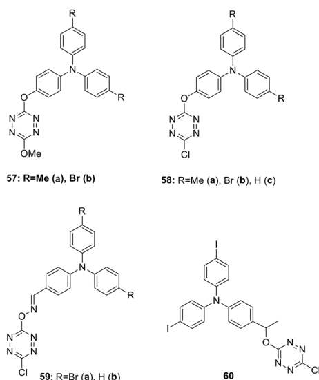
Fig. 4 Chemical structure of methoxy and chloro tetrazine derivatives 57–60 .
