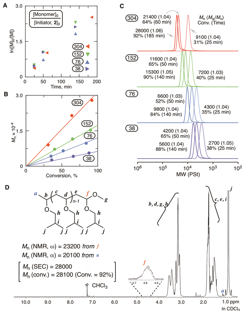
Fig. 2 \text{MgBr}_2 -catalyzed living cationic polymerizations of IBVE with 2 as an initiator: [\text{IBVE}]_0/[\text{2}]_0/[\text{MgBr}_2]_0/[\text{DTBMP}]_0 = 1520, 760, 380, \text{ or } 190/5.0/10/0.15 mM in toluene/ \text{Et}_2\text{O} (90/10 vol%) at 0^\circ\text{C} . (A) The first order kinetic plots, (B) the relationship between M_n s of the obtained poly(IBVE) and conversion, (C) SEC curves of the obtained poly(IBVE)s, and (D) ^1\text{H} NMR spectrum of poly(IBVE) obtained at 92% conversion for [\text{monomer}]_0/[\text{initiator}]_0 = 304 .
