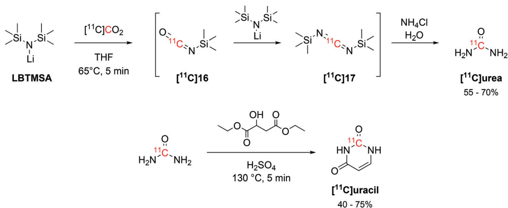
Scheme 9 Synthesis of ( ^{11}\text{C} )urea via the coupling of a silylamine precursor and ( ^{11}\text{C} ) \text{CO}_2 and subsequent condensation with diethyl malate for ( ^{11}\text{C} )uracil production. 57
