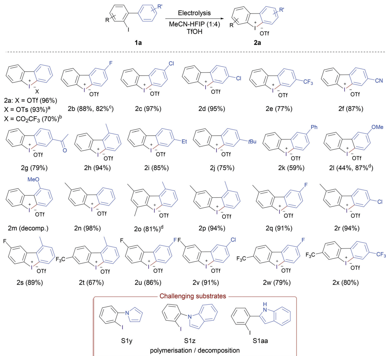
Scheme 1 Reaction scope of the electrochemical synthesis of cyclic diaryliodonium salts 2 . a \text{TfOH} replaced with \text{TsOH-H}_2\text{O} (2 equiv.). b \text{TfOH} replaced with \text{CF}_3\text{CO}_2\text{H} (5 equiv.). c Using substrate 1b' . d Obtained using Pt–Pt with alternating polarity.
