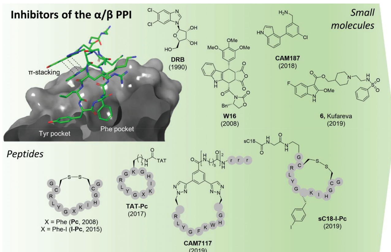
Fig. 9 CK2 inhibitors reported in chronological order and acting at the protein interface between the catalytic and regulatory subunit with the co-crystal structure of CK2 \alpha and CAM7117 shown on the left (PDB: 6Q4Q). The hydrophobic Tyr and Phe pockets key to binding are highlighted, alongside the \pi - \pi stacking interactions of the ligand. sC18 = H 2 N-GLRKRLKFRNKIKEK-NH 2 , 93 TAT = GRKKRRQRRRPPQ. 96 Compounds have been labelled as in the related papers. r = D-Arg.
