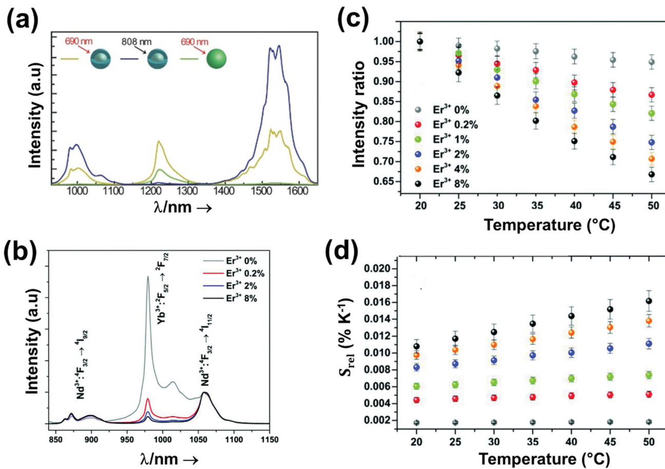
Fig. 28 (a) Room temperature emission spectra of simple core Er^{3+},Tm^{3+}, Yb^{3+}:LaF_3 under 690 nm excitation (green) and of active core@active shell Er^{3+},Yb^{3+}:LaF_3@Yb^{3+},Tm^{3+}:LaF_3 (concentrations of lanthanide ions Tm^{3+},Yb^{3+} and Er^{3+} are 10 mol%, 10 mol% and 2 mol%, respectively) under 690 (yellow) and 808 nm (blue) laser excitation. The green sphere and the grey core covered with a blue sphere represent the simple core and the active core@active shell, respectively. Reprinted with permission from ref. 240. Copyright 2017, Wiley-VCH Verlag GmbH & Co. KGaA. Effect of the Er^{3+} concentration on: (b) the intensity of the emissions, (c) the intensity ratio, and (d) S_{rel} on Tm^{3+},Yb^{3+}:SrF_2@Y^{3+}:SrF_2@Er^{3+},Nd^{3+},Yb^{3+}:SrF_2@Nd^{3+}:SrF_2 nanocrystals. (b)–(d) Adapted with permission from ref. 242. Copyright 2018, The Royal Society of Chemistry.
