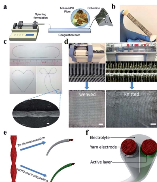
Fig. 7 (a) Schematic illustration of the spinning process of the MXene/PU fiber. (b) Digital photograph of fabricated MXene/PU fiber. Reproduced with permission. 120 Copyright 2020, Wiley-VCH. (c) Flexibility demonstration and SEM image of the yarn. (d) Demonstration of weavability and knittability. (e) Schematics of yarns electrodeposited with Zn and NCHO and (f) solid-state yarn battery. Reproduced with permission. 121 Copyright 2017, American Chemical Society.
