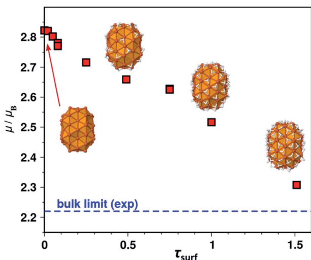
Fig. 4 Evolution of the magnetic moment per Fe atom of \text{B2-Fe}_{91}\text{H}_n as a function of \tau_{\text{surf}} .
