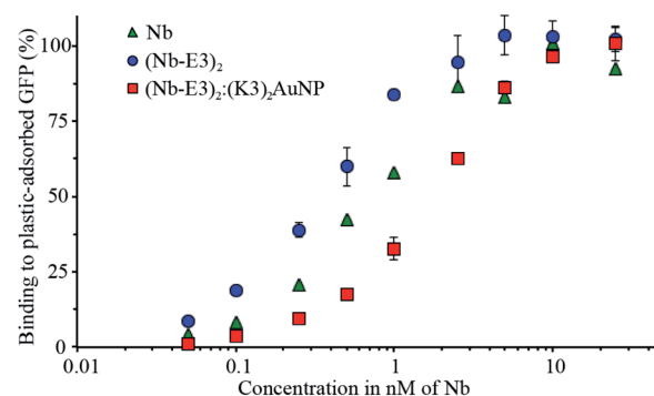
Fig. 5 Apparent binding abilities of the GFP-binding nanobody (green triangle), and the dimerized (Nb-E3) 2 (blue dot) and the non-covalent (Nb-E3) 2 ((K3) 2 AuNP assemblies (red square). The binding to GFP was determined using indirect ELISA analysis and plate-adsorbed GFP
