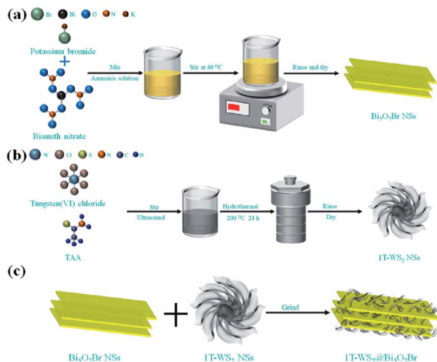
Scheme 1 Schematic route for the synthesis of (a) pure \text{Bi}_2\text{O}_5\text{-7Br} NSs, (b) 1T- \text{WS}_2 NSs and (c) 1T- \text{WS}_2 @ \text{Bi}_2\text{O}_5\text{-7Br} composites. Reprinted with permission from ref. 101 Copyright 2015, the American Chemical Society.
