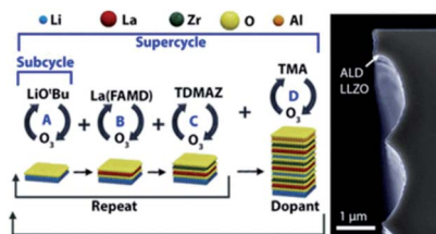
Fig. 6 Schematic representation of an ALD supercycle for the growth of Al-doped LLZO films and the corresponding TEM micrograph. 26
