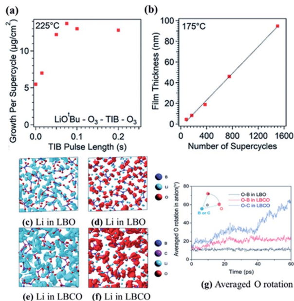
Fig. 16 Characterization of ALD film growth with an in situ quartz crystal microbalance, showing (a) saturation of the growth rate with increasing TIB pulse time, and spectroscopic ellipsometry showing (b) linearly increasing film thickness with the number of supercycles. (c–f) Iso-surfaces of the ionic probability densities evaluated from ionic trajectories calculated over 60 ps AIMD at 500 K. (g) Average oxygen rotational displacements in borate and carbonate anions during AIMD. The iso-surfaces are plotted using an isosurface value of 2P_0 ( P_0 represents the average probability density), for (c) Li in LBO, (d) O in LBO, (e) Li in LBCO, and (f) O in LBCO. (g) Averaged oxygen rotational displacements of LBO and LBCO during AIMD at 500 K. 47
