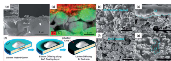
Fig. 8 Characterization of ALD ZnO coating to improve the surface wettability of garnet-type SSEs with molten lithium. Cross-sectional (a) SEM images and (b) elemental mapping of the garnet electrolyte coated with a 50 nm ALD ZnO layer. The inset of (a) shows a cross-sectional SEM image of the SSE/ZnO interface at higher magnification. (c) Schematic of the lithium diffusion process along the ZnO coating layer on the SSE surface. The cross-sectional SEM images of (d) the pristine and (e) the lithium infiltrated porous SSE with a porosity of 60–70%. (f) The cross-sectional SEM image of the porous garnet coated with a conformal ZnO surface layer using the ALD process. (g) The cross-sectional SEM images of a lithium infiltrated porous SSE with ZnO surface treatment, where almost all pores have been filled with Li metal. The Li metal area has been marked with a cyan dashed line. 28
