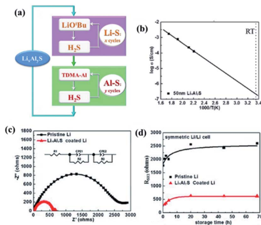
Fig. 14 (a) Schematic illustration of \text{Li}_x\text{Al}_x\text{S} ALD, (b) Arrhenius plot for temperature-dependent ionic conductivity measured using a 50 nm \text{Li}_x\text{Al}_x\text{S} film, (c) AC impedance spectra of Li/electrolyte/Li symmetric cells using both pristine Li and \text{Li}_x\text{Al}_x\text{S} -coated Li after 68 h storage, and (d) R_{\text{SEI}} of Li/electrolyte/Li symmetric cells versus storage time. 40
