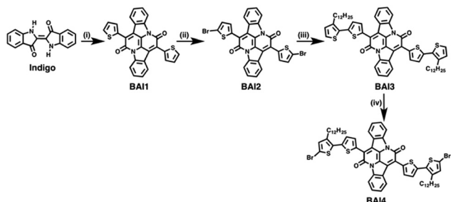
Scheme 2 Synthesis of BAI monomers. Reaction conditions: (i) 2-thienylacetyl chloride, xylene, 145^\circ\text{C} , 48 h, 38.5%; (ii) NBS, chloroform, rt, 15 h, 69.7%; (iii) 2-(trimethylstannyl)-3-dodecylthiophene, \text{Pd}(\text{PPh}_3)_4 , \text{P}(o\text{-tol})_3 , toluene, 100^\circ\text{C} , 4 days, 1.5%; (iv) NBS, chloroform, rt, 12 h, 87.1%.
