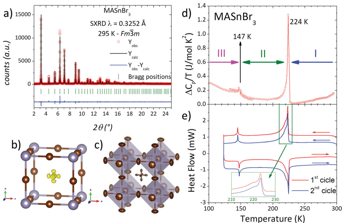
Fig. 1 (a) Observed (circles), calculated (full line) and difference (bottom) Rietveld profiles for \text{MASnBr}_3 from SXRd data at RT. (b) Octahedral framework including Sn and Br atoms, with DFM before MA incorporation. (c) Final cubic crystal structure after the Rietveld refinement at RT. (d) Heat capacity plotted as \Delta C_p/T vs. T . (e) First and second cycles of DSC curves. Inset shows an extended region of the most intense peak.
