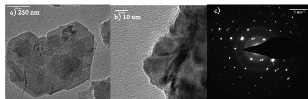
Fig. 2 TEM images (a) and (b). Diffraction of DPCOF spacing which corresponds to 2\theta 18-19^\circ . The CTEM image displays clear hexagonal symmetry and crystalline order which can be seen in DPCOF SAD (c) diffraction from (b).
