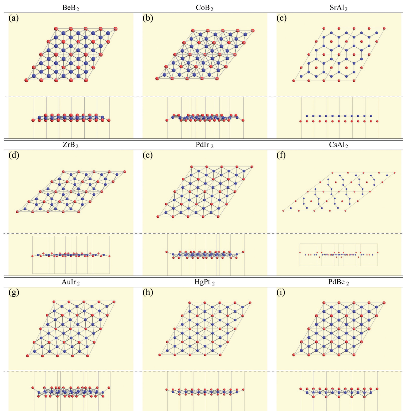
Fig. 8 Top and side views of 9 memory structures.
