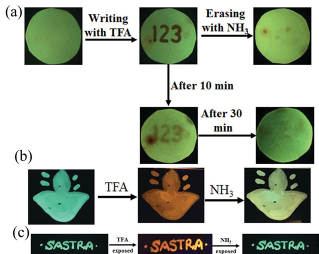
Fig. 9 Fabricating rewritable/self-erasable fluorescent platforms using 3-PMMA on (a) a filter paper, (b) symbol on a glass plate and (c) word writing on a glass plate ( \lambda_{\text{exc}} = 365 \text{ nm} ).
