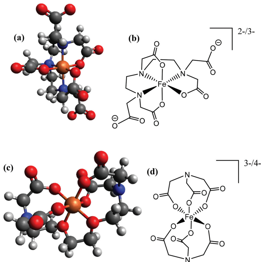
Fig. 8 Showing (a and c) energy minimised and (b and d) the equivalent skeletal structures of the (top) [Fe(DEPTA)] 2-/3- and (bottom) [Fe(NTA) 2 ] 3-/4- .
