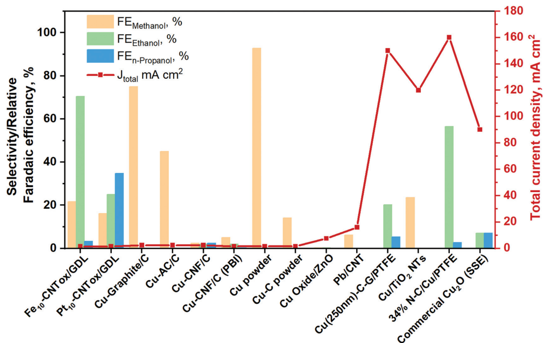
Fig. 13 Relative faradaic efficiencies and total current densities of the best catholyte-free EC \text{CO}_2\text{R} electrocatalysts towards methanol, ethanol and n -propanol production. Authors with data taken from ref. 131 and 133–140.
