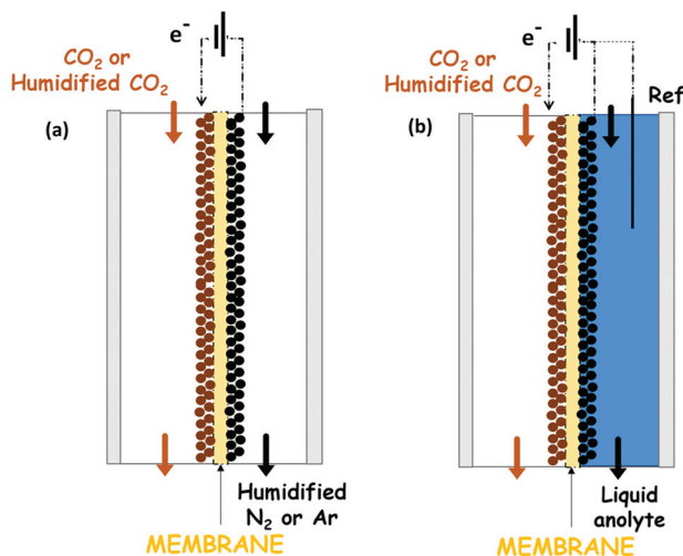
Fig. 12 Representation of the most popular catholyte-free configuration, in continuous flow, for the electrochemical \text{CO}_2 reduction: (a) solvent-less cell configuration, (b) liquid anolyte cell configuration.
