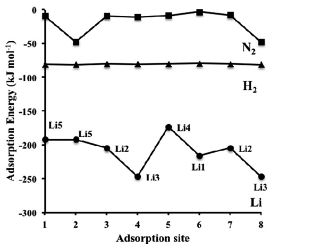
Fig. 8 Dispersion-corrected (revPBE-D3) adsorption energies of Li (circles), H 2 (triangles) and N 2 (squares) over the symmetry unique adsorption sites on \eta -Mn 3 N 2 depicted in Scheme 1 (for H 2 and N 2 ). The data for Li corresponds to the adsorption site configuration depicted in Scheme 2. Lines connecting the data points have been drawn to guide the eye.
