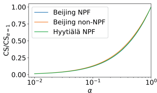
Fig. 6 Ratio of the condensation sink (CS) of sulfuric acid (SA) with varying mass accommodation coefficients ( \alpha ) to the CS assuming \alpha = 1 . CS values have been determined from three different particle number size distributions: median NPF size distributions from Beijing, China and Hyytiälä, Finland and median non-NPF size distribution from Beijing (see Section 2.2).
