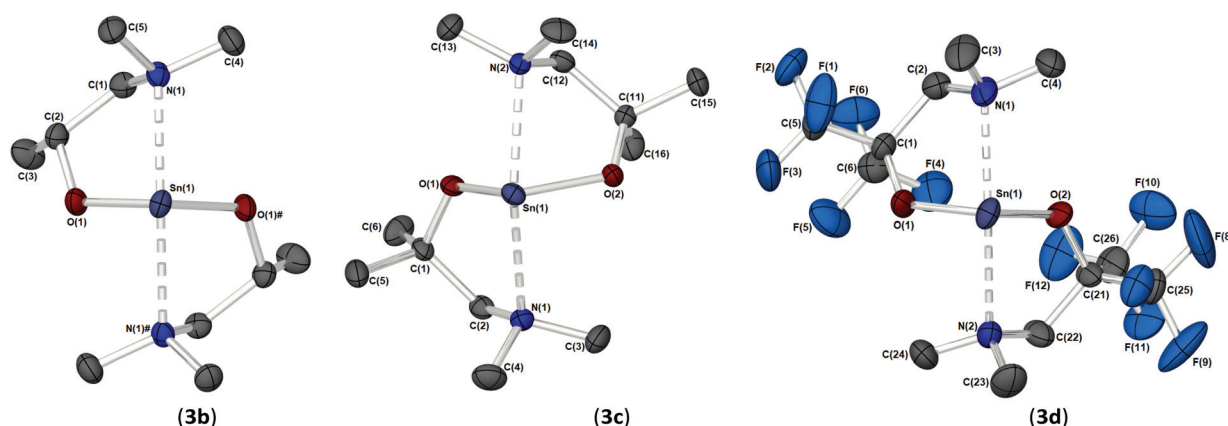
Fig. 5 The solid-state molecular structures of (a) [Sn{dmamp} 2 ] ( 3b ), (b) [Sn(dmamp) 2 ] ( 3c ) and (c) [Sn{Fdmamp} 2 ] ( 3d ). Thermal ellipsoids are shown at 50% probability and H-atoms are omitted for clarity. The symmetry equivalent atoms in 3b are generated by the operator: # 1 - X, Y, \frac{1}{2} - Z.
